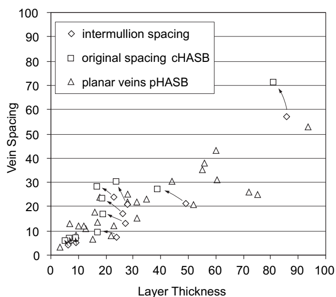
Fig. 10. S/T - versus S_0/T_0 relationship of intermullion veins for some examples from the cHASB, compared to the S/T relationship of planar veins from the pHASB.
