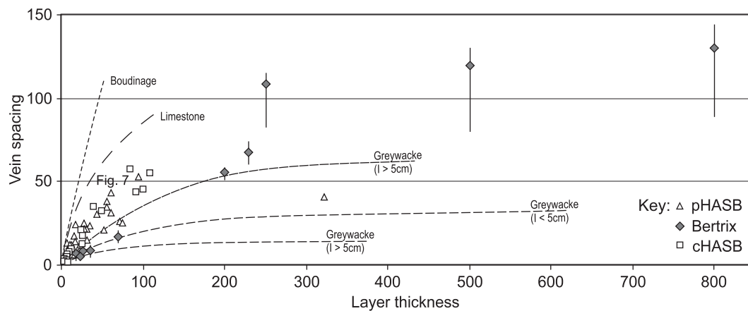
Fig. 9. Vein spacing (in cm) versus layer thickness (in cm) relationship for quartz veins in thick metasedimentary multilayer sequences (data from Bertrix; cHASB). Compared to fracture spacing (data from Ladeira and Price, 1981), vein spacing is wider in thick units although a lack of measurements may obscure these results. See text for discussion. Axes have a different scale.
