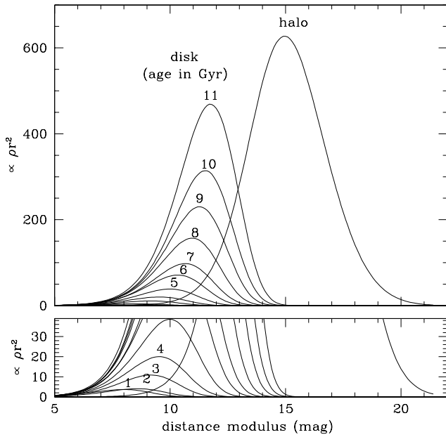
Fig. 5. Distribution of stellar distance moduli in the simulation corresponding to our initial calibration, in a conic beam towards the NGP. This is shown for 11 disc components of increasing age – at steps of 1 Gyr, as labelled – and for the halo. The top panel shows all the curves, whereas the bottom one expands the vertical axis in order to detail the profiles for ages younger than 5 Gyr. It can be noticed that younger disc components are found at lower mean distances (peaking from say \mu_0 = 8 to 12 as the age increases), whereas the halo stars are found with a nearly-Gaussian distribution of \mu_0 which peaks at about 15. The characteristic shapes of these distributions result from two competing trends in Eq. (1): the quadratic increase of the geometrical factor r^2 , and the almost-exponential decrease of the density \rho with distance to the Galactic Plane.
