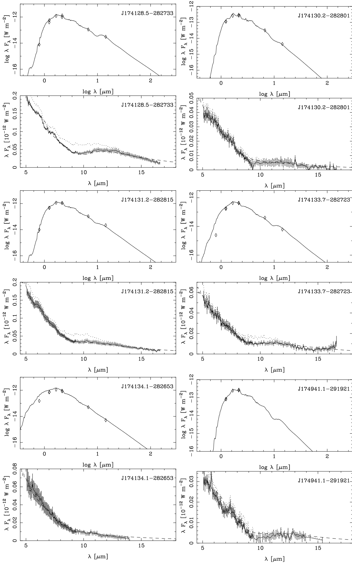
Fig. 3. Model fits to the DENIS, 2MASS and ISOGAL photometry and spectra. Continued
