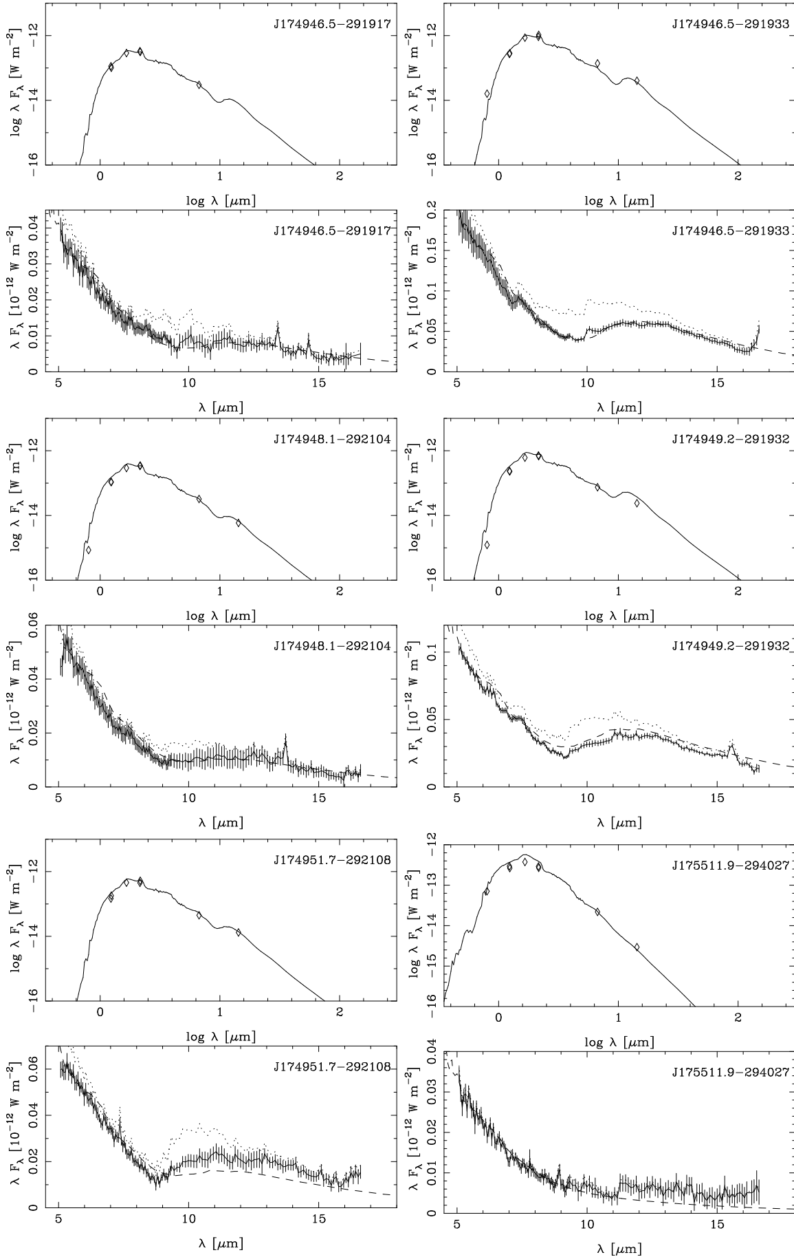
Fig. 5. Model fits to the DENIS, 2MASS and ISOGAL photometry and spectra. Continued
