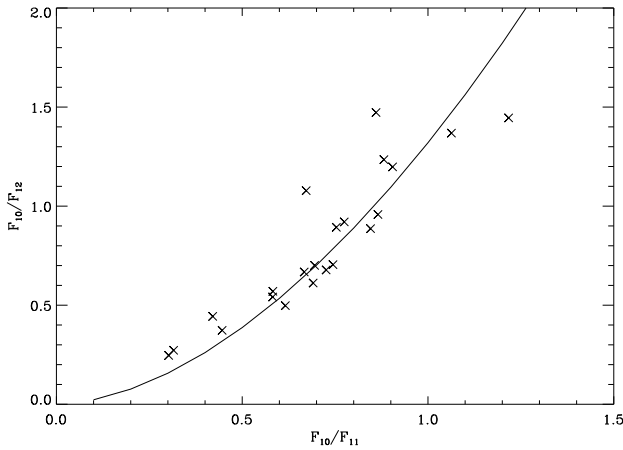
Fig. 8. The silicate dust sequence, as defined in Sloan & Price (1995). The power law was a fit to their sample and is also a good representation for the dust features seen in our sample.
