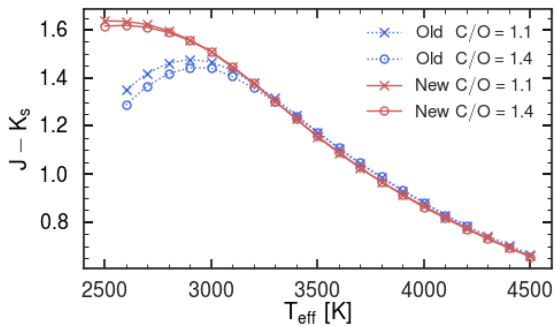
Figure 10. Predicted J - K_s colour as a function of effective temperature calculated from COMARCS models with a surface gravity of \log(g \text{ [cm/s}^2]) = 0.0 , a stellar mass of M = 1 M_\odot and solar abundances except for carbon. Two C/O ratios (1.1 – crosses, 1.4 – circles) are shown. The results are based on the standard grid by Aringer et al. (2016, old, blue dotted lines) and on computations with the new opacities for \text{C}_2\text{H}_2 and \text{C}_2 (new, red solid lines).
