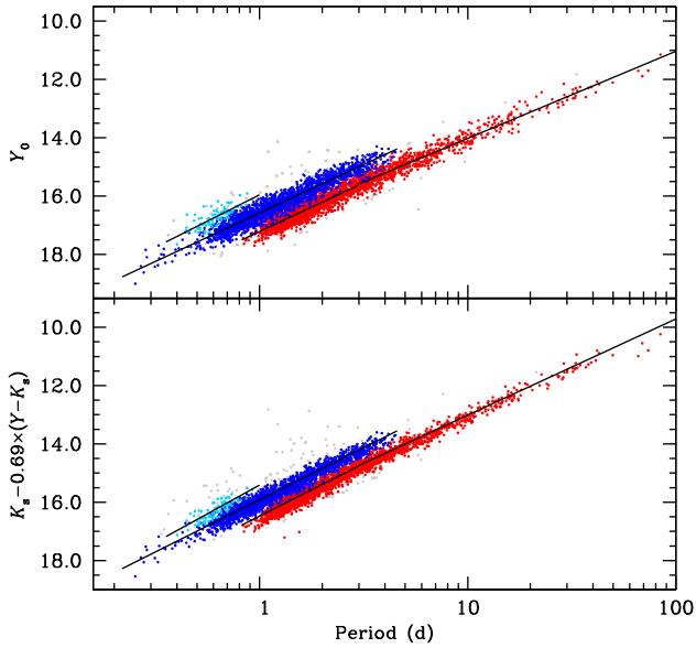
Figure 4. PL(Y) and PW(K_s, Y) relations for the SMC CCs investigated in this paper. F, IO and 2O pulsators are shown as red, blue and light blue filled circles, respectively. The grey filled circles show objects excluded from the analysis because they deviate more than 3.5\sigma from the best fits to the data represented by solid lines.
