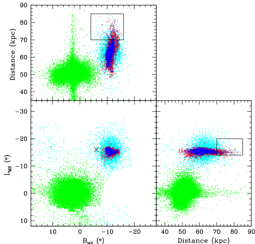
Figure 17. Position of LMC and SMC RR Lyrae as well as of young and old CCs in the SMC (same colour coding as in Fig. 16) in Magellanic coordinates (bottom-left) or Magellanic longitude/latitude versus distance (bottom-right and top-left, respectively). This figure is similar to fig. 8 of Diaz & Bekki (2012), whose prediction can be directly compared. The approximate location of the predicted Counter-Bridge are shown with a diagonal cross (centre) in the bottom-left panel and with boxes in the top-left and bottom-right panels. The colour code of the data points is the same as in Fig. 16.
