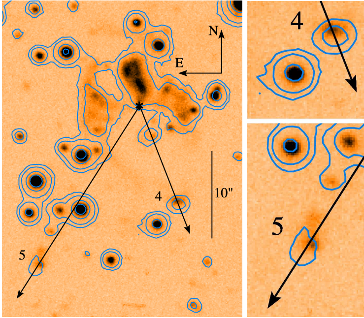
Figure 1. The expansion of the ejecta from the 1670 event in CK Vul. The negative image shows H \alpha observations from 1991 (Naylor et al. 1992), the contours are H \alpha observations from 2004 taken from the IPHAS survey (Drew et al. 2005). The asterisk marks the position of the radio source. Knots 4 & 5 are enlarged on the right.
